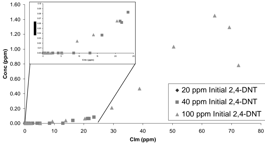
Figure 4.29 4A2NT effluent concentration vs. C_{Im} for differing initial concentrations of 2,4-DNT, 1 mMol formic acid, pH = 4.0
