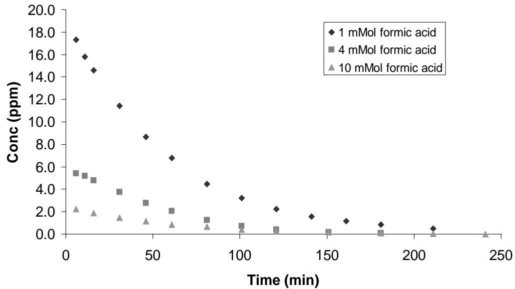
Figure 4.13b 2,4-DNT effluent concentration vs. time for differing concentrations of formic acid, 20 ppm initial 2,4-DNT concentration, pH = 6.0 - 6.4
