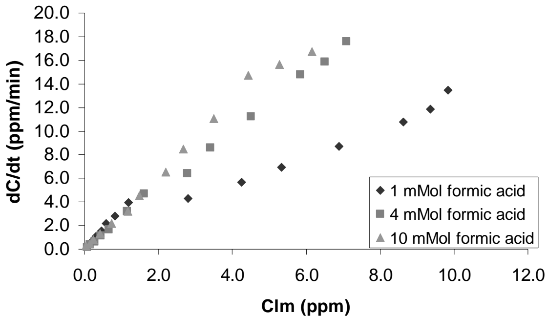
Figure 4.15 2,4-DNT degradation rate vs. C_{1m} for differing concentrations of formic acid, 20 ppm initial 2,4-DNT concentration, pH = 4.0
