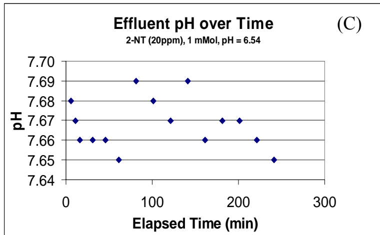
Figure A.4a Exp #4 – 20 ppm 2-NT, 1mMol Formic acid, pH = 6.54 (A) Influent vs. Effluent 2-NT Concentration (B) Removal vs. Clm (ppm) (C) Effluent pH vs. Time
