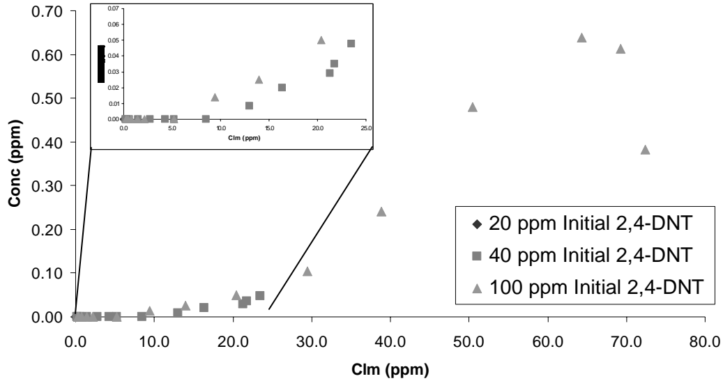
Figure 4.28 2A4NT effluent concentration vs. C_{Im} for differing initial concentrations of 2,4-DNT, 1 mMol formic acid, pH = 4.0
