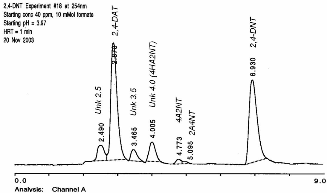
Figure 4.34 HPLC response curve from Experiment #18 showing all known and unknown byproducts
