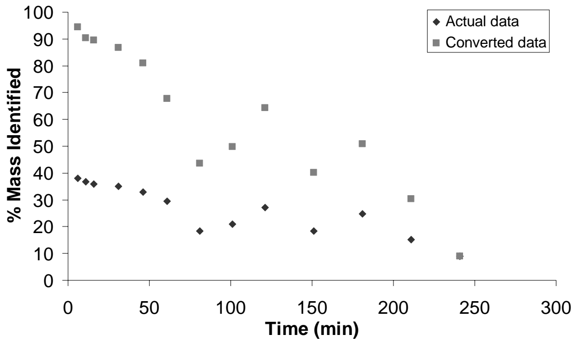
Figure 4.33 % mass identified vs. time for Experiment #22 with actual and converted 2,4-DAT mass data
