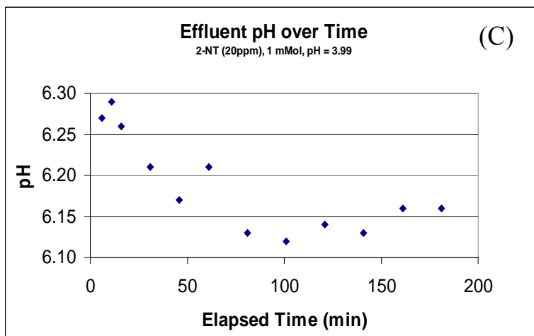
Figure A.2a Exp #2 – 20 ppm 2-NT, 1mMol Formic acid, pH = 3.99 (A) Influent vs. Effluent 2-NT Concentration (B) Removal vs. CIm (ppm) (C) Effluent pH vs. Time
